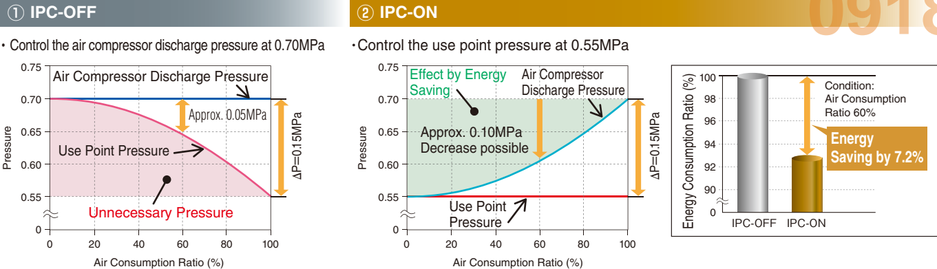
Graph of pressure change (Theoretical values)
