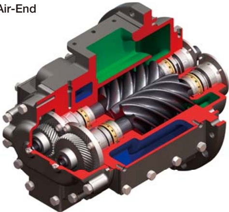
Air-End
